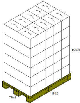
EPAL ( mm 1200 x 800 x 144 )
